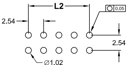
Recommended PCB Layout Top View (Tolerance ±0.05)
